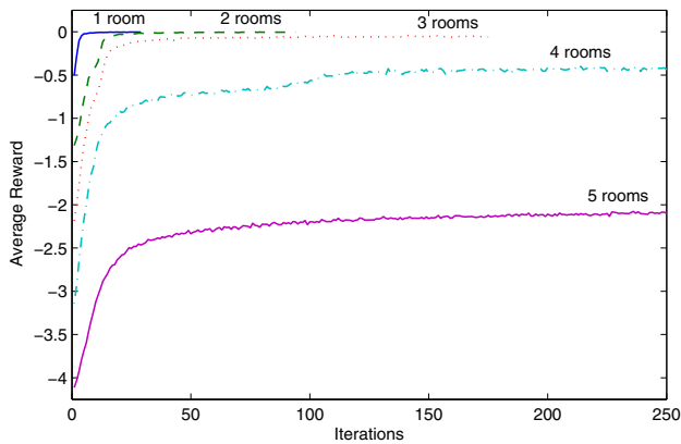
Fig. 4. Safety problem ( n = 1, \dots, 5 ): reward evolution as a function of the algorithm iterations.
