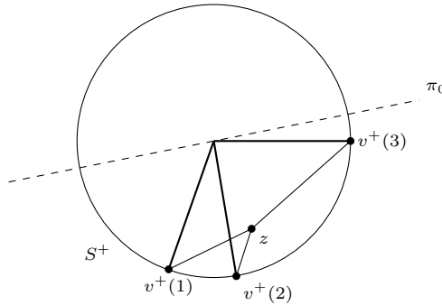
Fig. 3. The restriction of currents W and Z in B_1^{n+1} : in this example, the modulus is p = 3 and the multiplicities m^+(j) are all equal to 1. The current W is represented by the thicker lines connecting the points v^+(j) to the center of the circle, while the current Z is represented by the lighter lines connecting the points v^+(j) to the point z .
