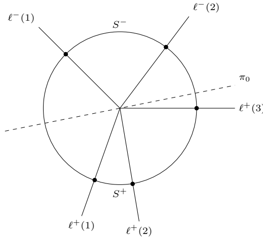
Fig. 2. The two hemispheres S^+ and S^- and the rays \ell^+(j) and \ell^-(l) . The points v^+(j) and v^-(l) are the intersections of the rays with the appropriate hemisphere.
