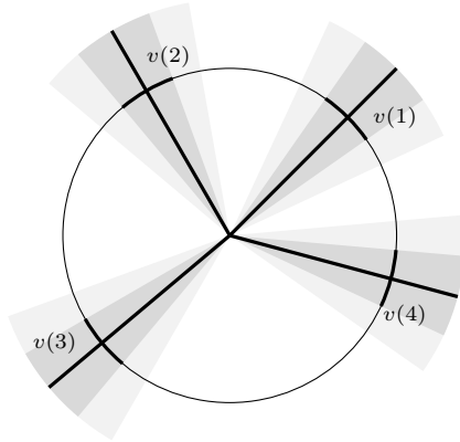
Fig. 7. A visual illustration of the map F . In the nonshaded areas F takes the constant value 0. In each of the four darker shaded areas F(x) is the unique point in the central halfline such that |F(x)| = |x| (hence each thick arc is mapped into its middle point v(i) ). In the remaining lighter shaded areas the map F is extended to be Lipschitz, while still taking values in the nearest thick halfline.
