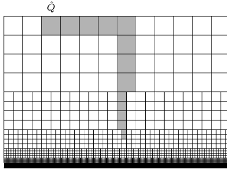
Fig. 5. An example of \mathscr{W}(Q_0) .
