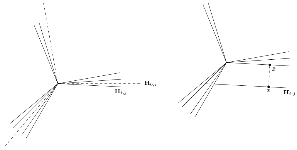
Fig. 6. The picture on the left shows the books \mathbf{S}_0 (dashed lines) and the book \tilde{\mathbf{S}} (solid lines). The page \mathbf{H}_{0,i} is pictured horizontal and the page \mathbf{H}_{i,j} is the “lowest page” of \tilde{\mathbf{S}} among those close to \mathbf{H}_{0,i} . The angle formed between q_0 and \mathbf{H}_{0,i} is larger than a geometric constant (depending only on \mathbf{S}_0 ) and much larger than the angle between \mathbf{H}_{0,i} and \mathbf{H}_{i,j} . The picture on the right shows \mathbf{H}_{i,j} , the translated book q_0 + \tilde{\mathbf{S}} and a point x \in \mathbf{H}_{i,j} with the property that |x - q_0| \geq C|x_0| for a suitable constant. Observe that \text{dist}(x - q_0, \tilde{\mathbf{S}}) = \text{dist}(x, q_0 + \tilde{\mathbf{S}}) = |\bar{x} - x| , where \bar{x} is the point on q_0 + \tilde{\mathbf{S}} closest to x . Note that \bar{x} must belong to q_0 + \mathbf{H}_{i,j} and \bar{x} - x must be orthogonal to it, in particular |x - \bar{x}| = |\mathbf{p}_{\mathbf{H}_{i,j}^\perp}(q_0)| .
