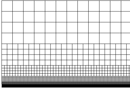
Fig. 4. The Whitney decomposition of [0, 2] \times [-2, 2]^{m-1} . In the above example the parameter M equals 2.
